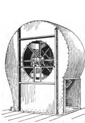
FIG. 28.—Full housed steel plate fan. Left-hand bottom horizontal discharge.
